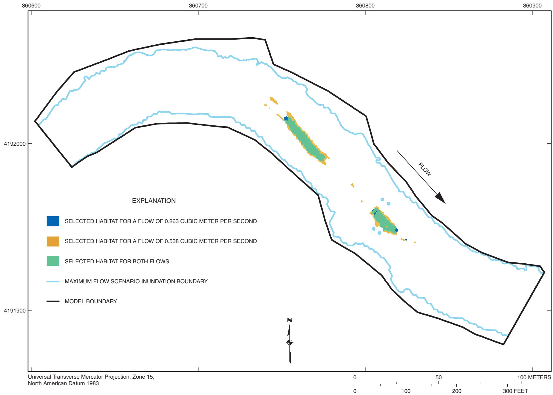
Figure 1-1. Selected habitat area distribution for habitat category 1 (suckermouth minnow) at flows of 0.263 and 0.538 cubic meter per second at Marmaton River site M1.
